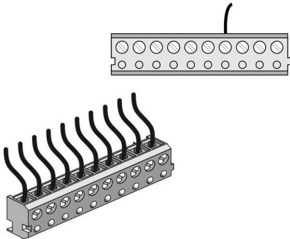
Fig.8 Connecting wire
