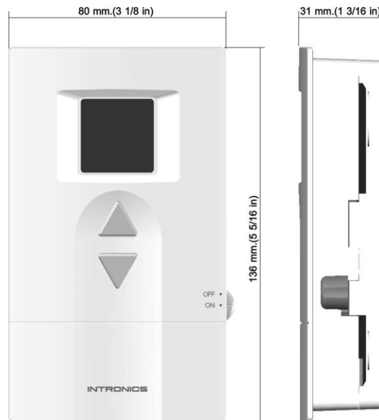
Fig.2 Dimensions
