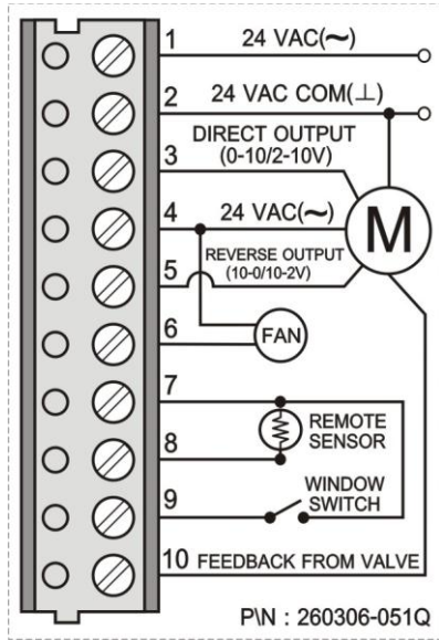
Fig.7 Wiring diagram
